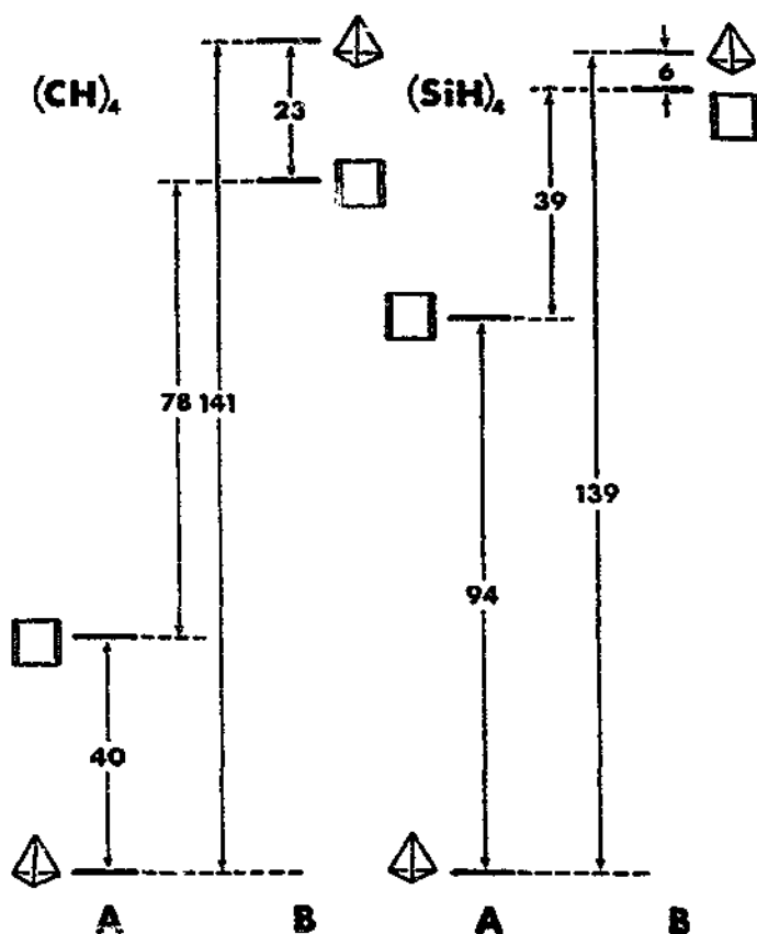
Fig. 6. Relative isomer energies (kcal mol -1 ) as determined by A, the bond additivity model and energy differences 2\Delta of average bond energies; and B, by ab initio calculations of total molecular energies.
