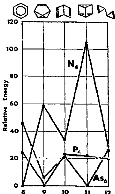
Fig. 8. Relative energies (kcal mol -1 ) of N 6 , P 6 , and As 6 analogs of the valence isomers of benzene as determined by ab initio calculations.
