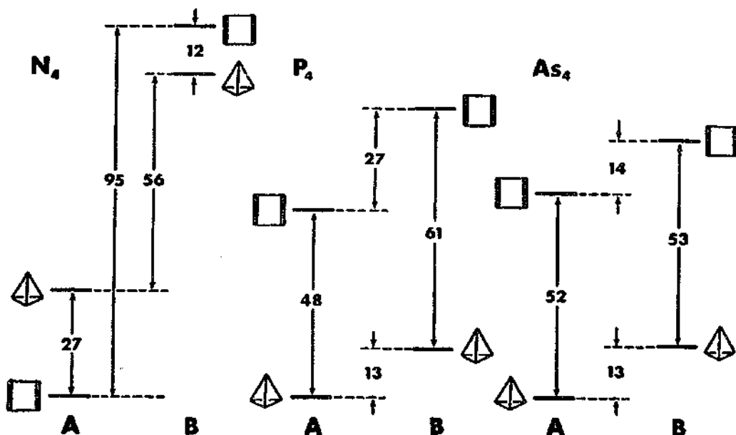
Fig. 5. Relative isomer energies ( \text{kcal mol}^{-1} ) as determined by A, the bond additivity model and energy differences 2\Delta of average bond energies; and B, by ab initio calculations of total molecular energies.
