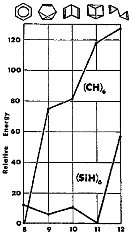
Fig. 7. Relative energies ( \text{kcal mol}^{-1} ) of the valence isomers of benzene as established by ab initio calculations.
