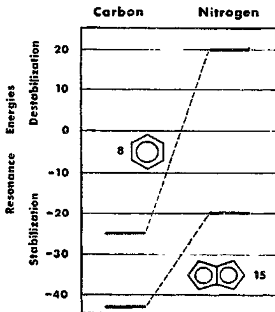
Fig. 11. Resonance energies ( \text{kcal mol}^{-1} ) for aromatic hydrocarbon and nitrogen clusters. Resonance stabilization of the hydrocarbons is much greater than that for the hypothetical nitrogen analogs. The energy gap between 8 and 15 is much larger for nitrogen clusters than for the hydrocarbons.
